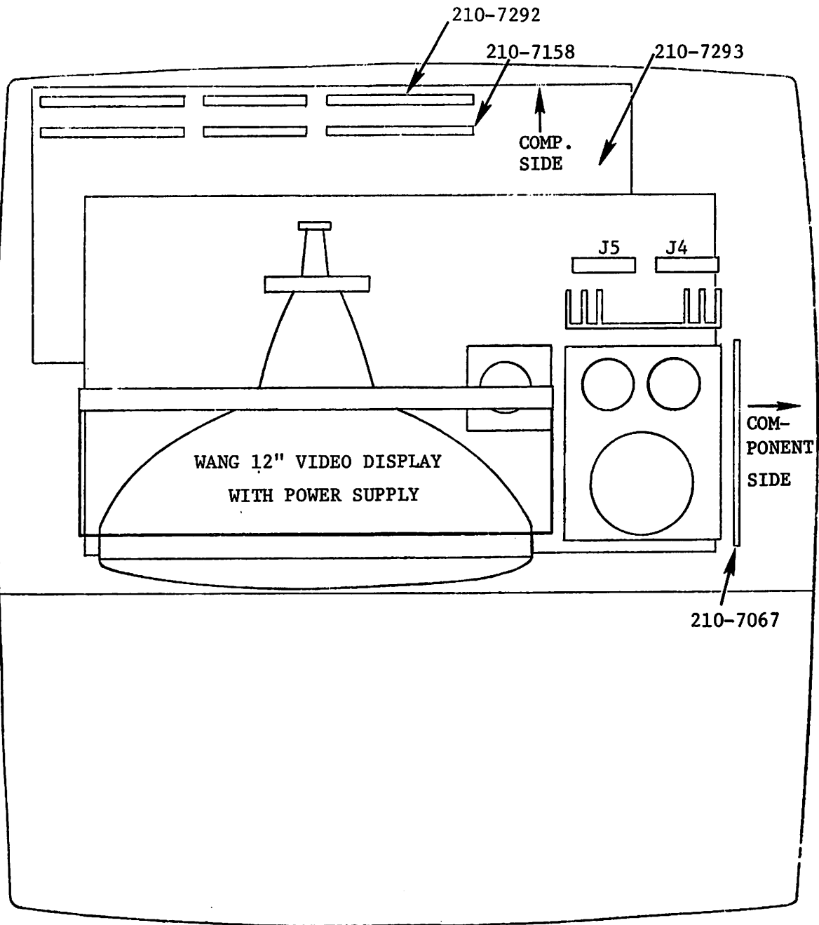
MODEL 2236 CHASSIS LAYOUT
