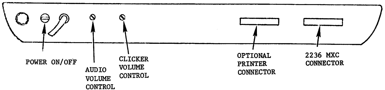
MODEL 2236 REAR PANEL
