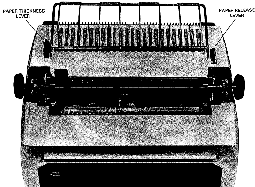
Figure 1-4. Platen Levers
